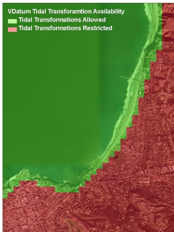
Figure 5.7. Illustrated are the areal extents of where VDatum allows/restricts tidal datum transformations.
